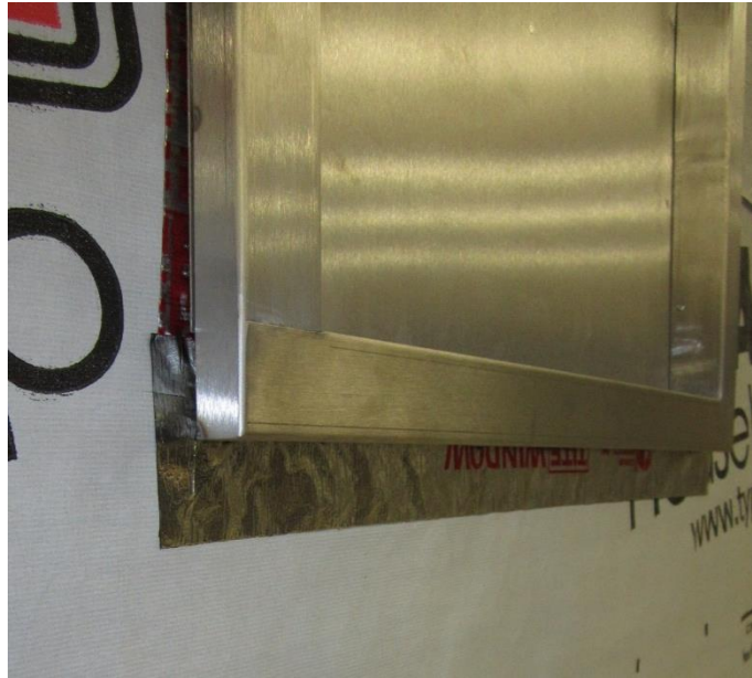
Ice & Water shield Placed Under Metal Edges
